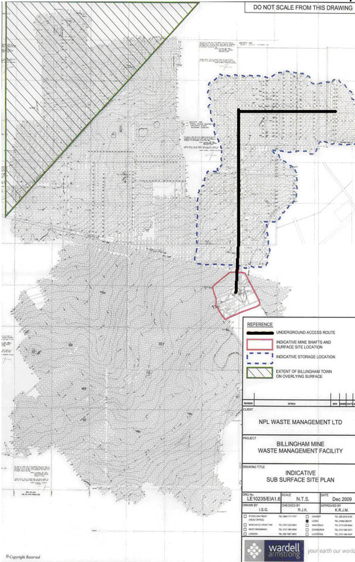
Indicative Sub Surface Site Plan
